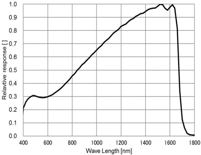
SWIR spectral response curve
